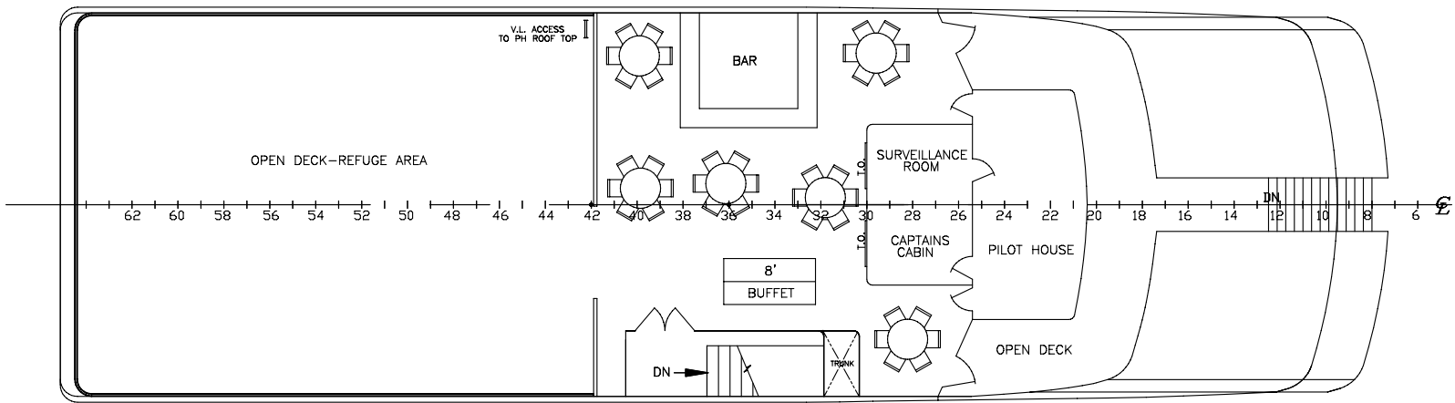
02 DECK
