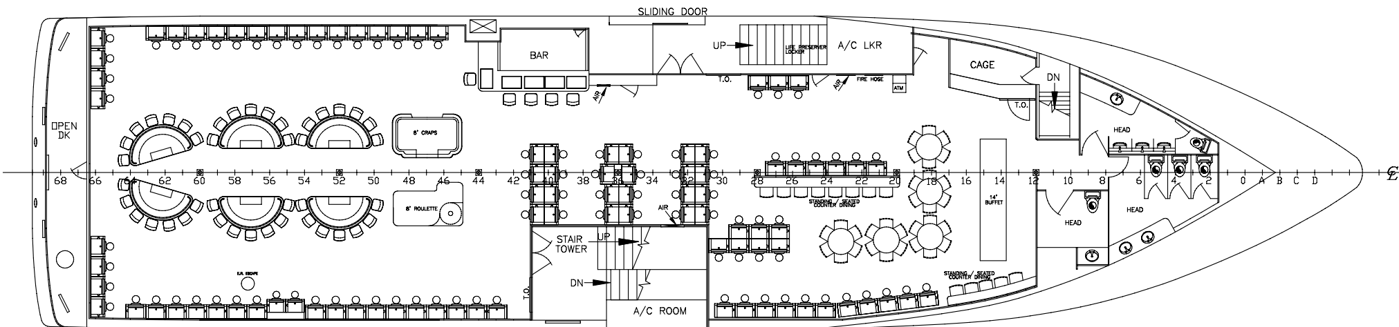
MAIN DECK
