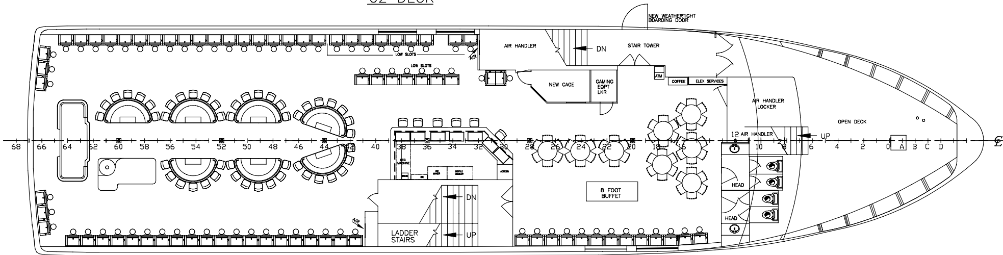
01 DECK
